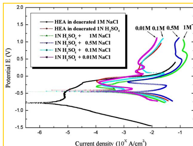
Fig. 12. Anodic polarization curves for HEA obtained in deaerated 1 N \text{H}_2\text{SO}_4/\text{X} NaCl ( \text{X} = 0\text{--}1\text{ M} ) solutions at room temperature ( \sim 25^\circ\text{C} ).
