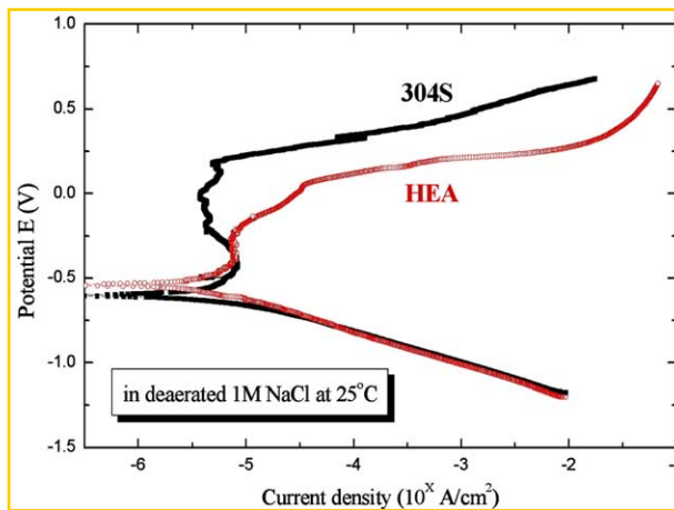
Fig. 8. Comparisons of the anodic polarization curves for the HEA and 304S in deaerated 1 M NaCl solution at room temperature (~25 °C).
