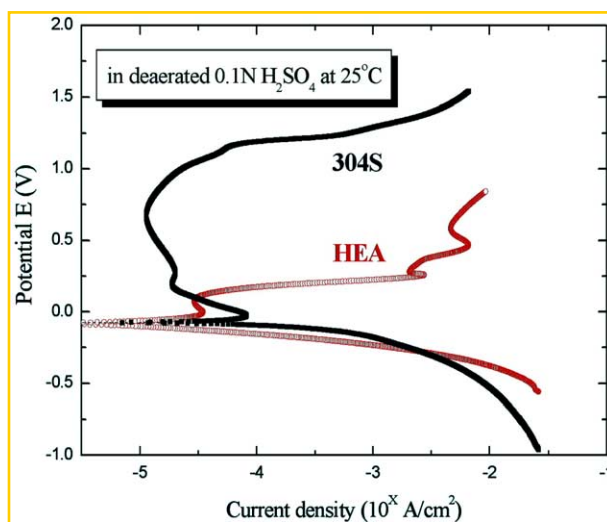
Fig. 10. Comparisons of the anodic polarization curves for the HEA and 304S in deaerated 0.1 N \text{H}_2\text{SO}_4 at room temperature ( \sim 25^\circ\text{C} ).
